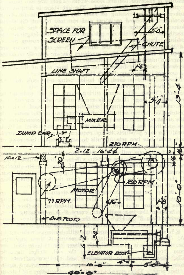
FIG. 118—PART ELEVATION, SHOWING ELEVATING MACHINERY, PLANT NO. 6
